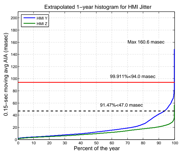
Figure 10: HMI Jitter
