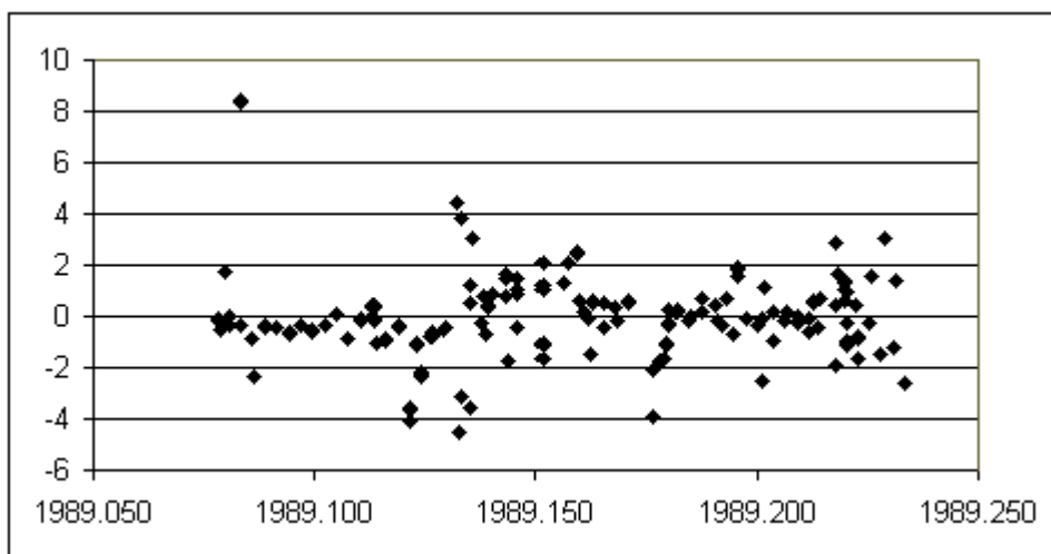
Fig. 11. Residuals for the SC Phobos-2 range rates. Time is in year fractions are on the abscissa axis, the ordinate axis in sm/sec.
