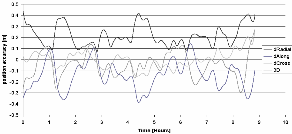
3D position accuracy with Rokar receiver
