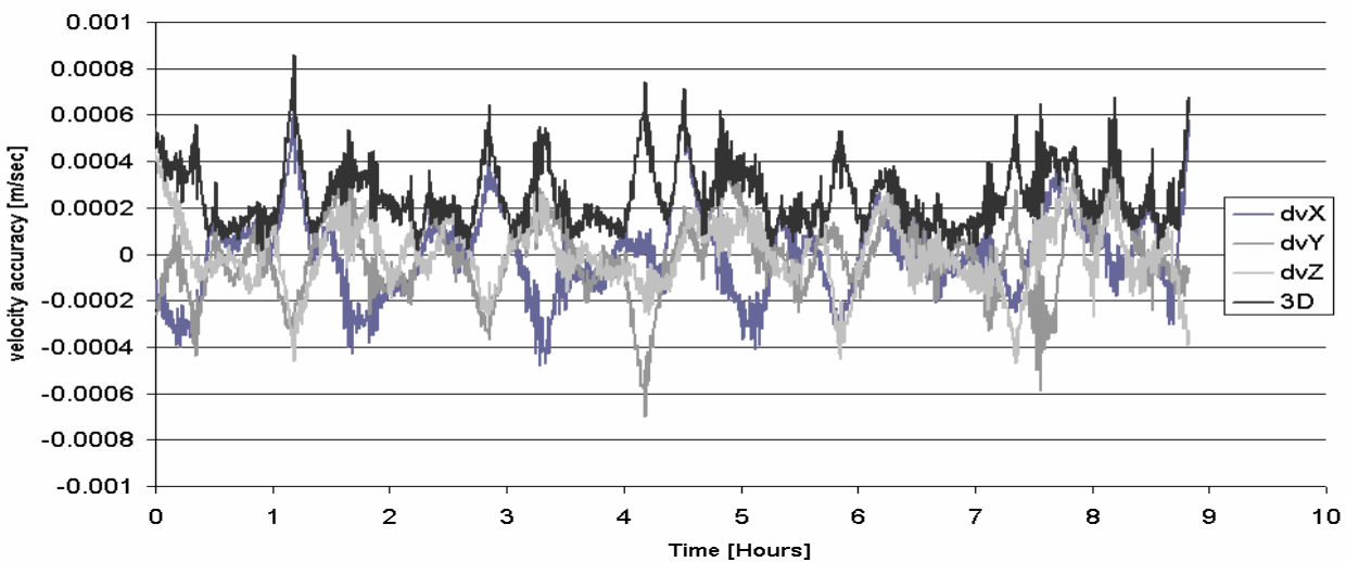
3D velocity accuracy with Rokar receiver
