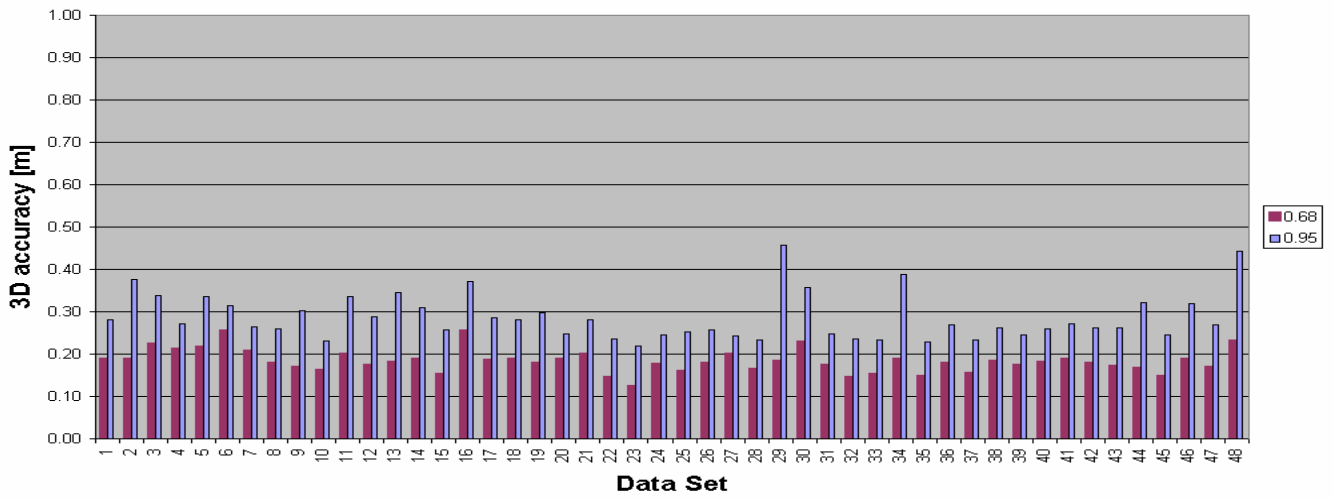
3D Accuracy - full GPS constellation
