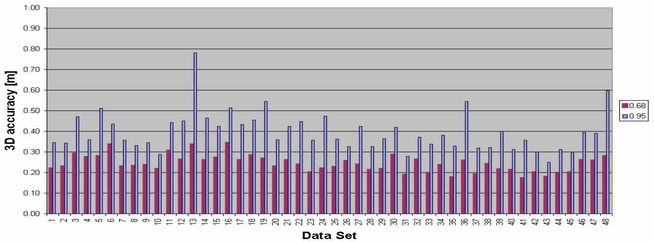
3D Accuracy - Inferior GPS constellation
