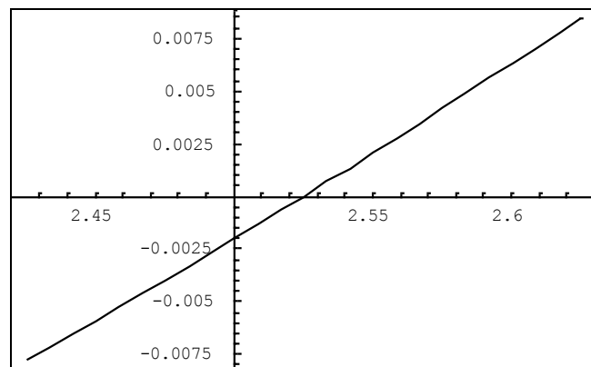
Figure 5. Variation in Inclination (rad) for r_p = 1.5 r_J and v_p = 4.5
