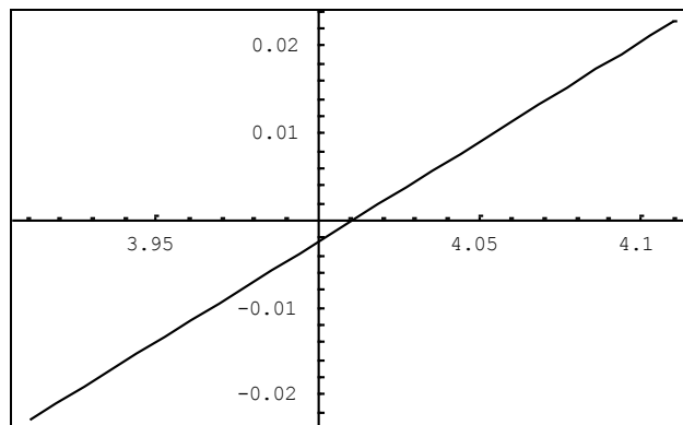
Figure 14. Variation in Velocity for r_p = 5.0 r_J and v_p = 4.5
