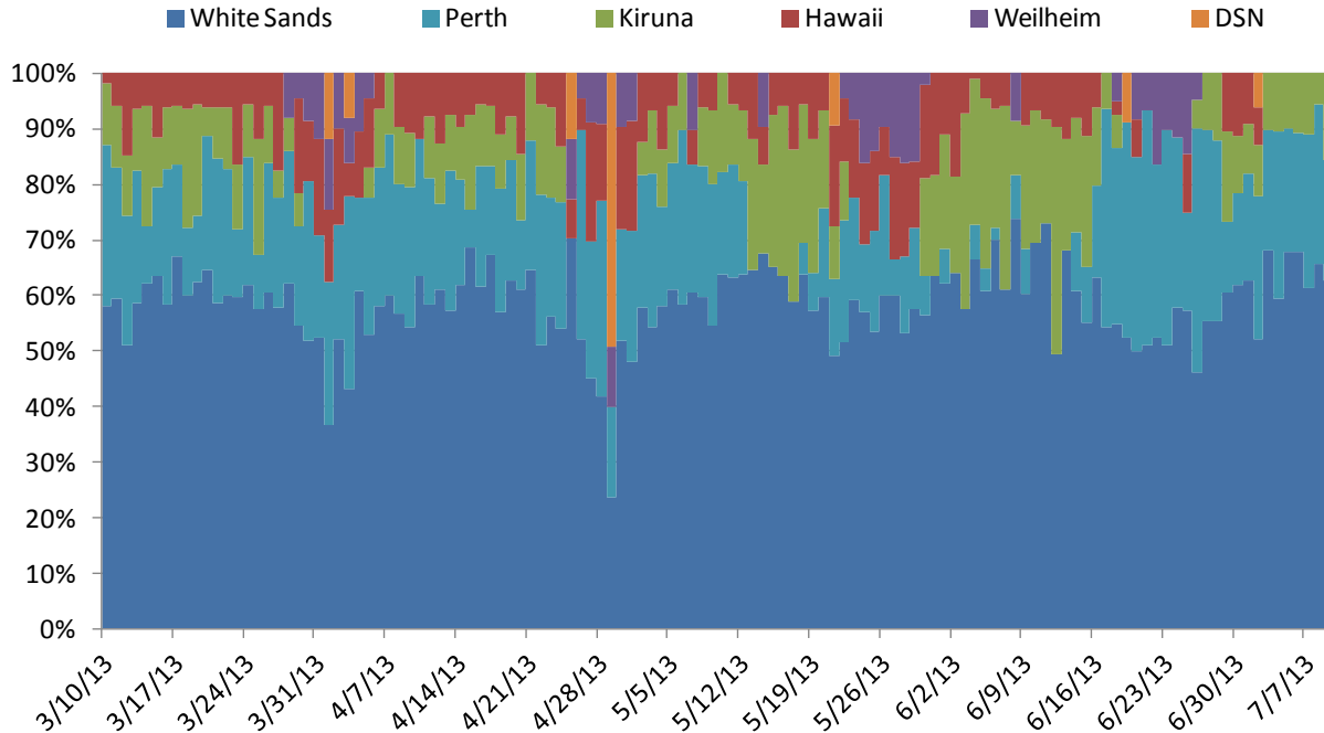
Figure 1. LRO tracking by station, as a fraction of total tracking
