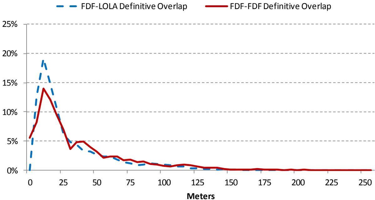
Figure 13. Distribution of total position difference between LOLA and FDF solutions using GSFC-GRAIL-270, and the FDF definitive overlap differences
