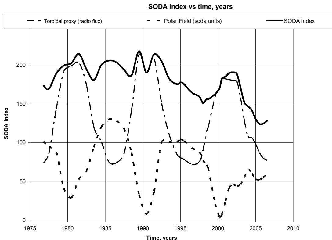
Figure 5. The SODA index is a composite index allowing us to monitor the "buried magnetic flux" present in the Sun's ever-changing dynamo.
