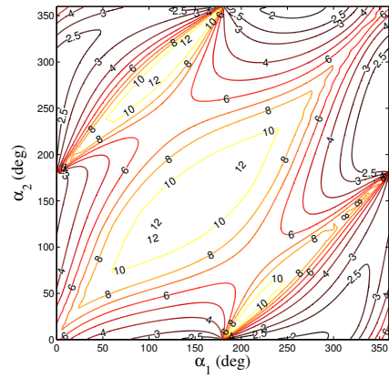
Figure 8: Contour-map of impulse function \Delta V_{tot} (km/s) necessary to reach GEO. Initial orbit O_I : p_1 = 22000 km, e_1 = 0.5^\circ , i_1 = 25^\circ , \Omega_1 = 0^\circ , \omega_1 = 150^\circ .
