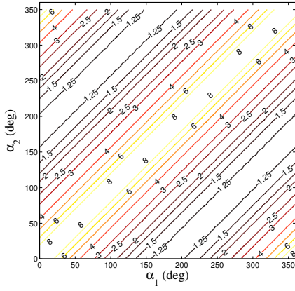
Figure 3: Contour-map of the impulse function \Delta V_{tot} (km/s) necessary to reach GEO. Initial orbit O_I : p_1 = 22000 km, e_1 = 0^\circ , i_1 = 0^\circ , \Omega_1 = 0^\circ , \omega_1 = 0^\circ .
