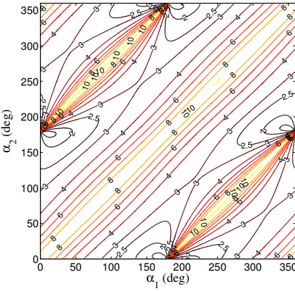
Figure 5: Contour-map of impulse function \Delta V_{tot} (km/s) necessary to reach GEO. Initial orbit O_I : p_1 = 22000 km, e_1 = 0^\circ , i_1 = 20^\circ , \Omega_1 = 0^\circ , \omega_1 = 0^\circ .
