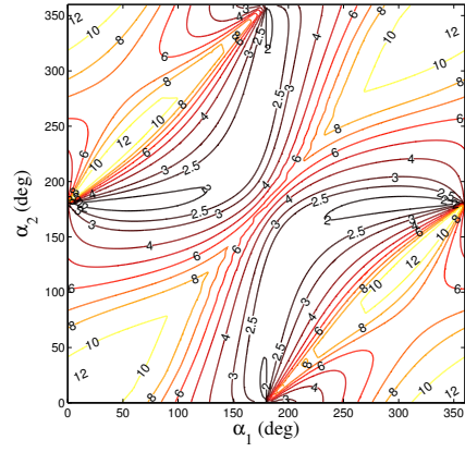
Figure 6: Contour-map of impulse function \Delta V_{tot} (km/s) necessary to reach GEO. Initial orbit O_I : p_1 = 22000 km, e_1 = 0.5^\circ , i_1 = 25^\circ , \Omega_1 = 0^\circ , \omega_1 = 0^\circ .
