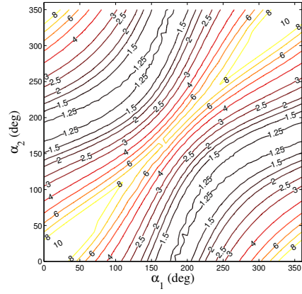
Figure 4: Contour-map of impulse function \Delta V_{tot} (km/s) necessary to reach GEO. Initial orbit O_I : p_1 = 22000 km, e_1 = 0.25^\circ , i_1 = 0^\circ , \Omega_1 = 0^\circ , \omega_1 = 0^\circ .
