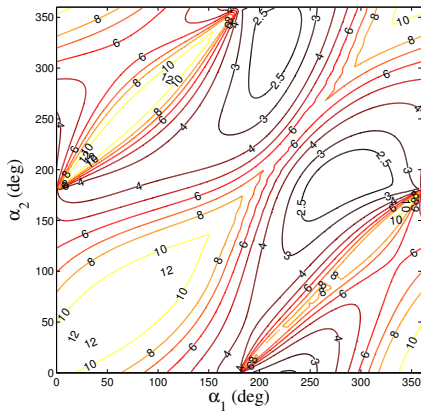
Figure 7: Contour-map of impulse function \Delta V_{tot} (km/s) necessary to reach GEO. Initial orbit O_I : p_1 = 22000 km, e_1 = 0.5^\circ , i_1 = 25^\circ , \Omega_1 = 0^\circ , \omega_1 = 60^\circ .
