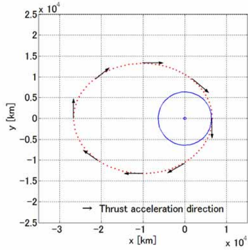
Fig.10 Optimum steering law for minimum \dot{a} (Inertial coordinate system)
