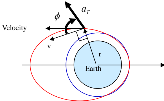
Fig.4 Definition of angle of thrust
