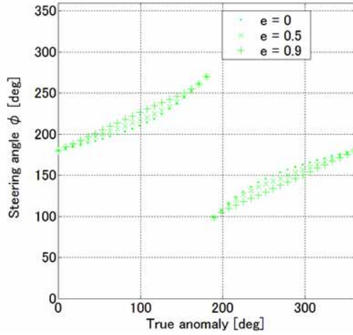
Fig.14 Optimum steering law for minimum \dot{r}_a ( a = R_e + 200 )
