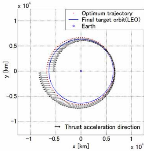
Fig.5 Optimum trajectory in quasi circular orbit (Inertial coordinate system)
