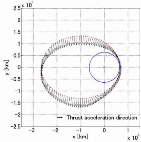
Fig.13 Optimum steering law for minimum \dot{e} (Inertial coordinate system) ( a = 16578, e = 0.60321 )
