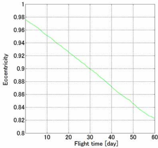
Fig.17 Change of eccentricity using steering law for 60 days
