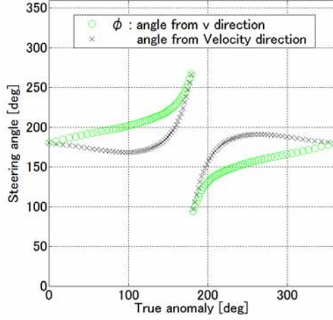
Fig.8 Optimum thrust steering angle profile
