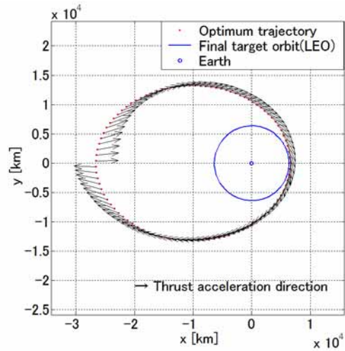
Fig.7 Optimum trajectory in elliptic circular orbit (Inertial coordinate system)
