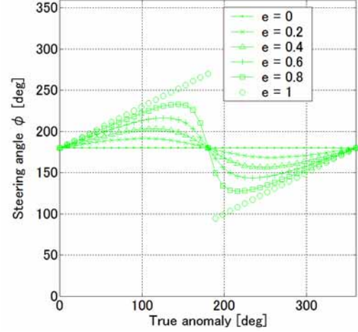
Fig.9 Optimum steering law for minimum \dot{a}
