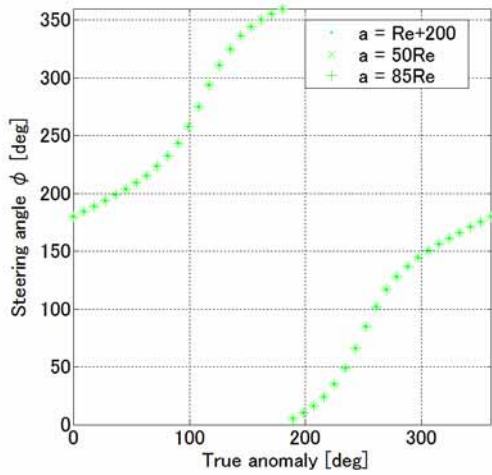
Fig.12 Optimum steering law for minimum \dot{e} ( e = 0.5 )
