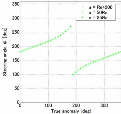
Fig.15 Optimum steering law for minimum \dot{r}_a ( e = 0.5 )
