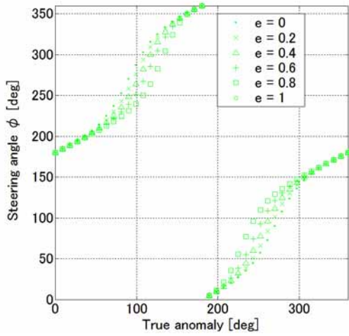
Fig.11 Optimum steering law for minimum \dot{e} ( a = R_e + 200 )
