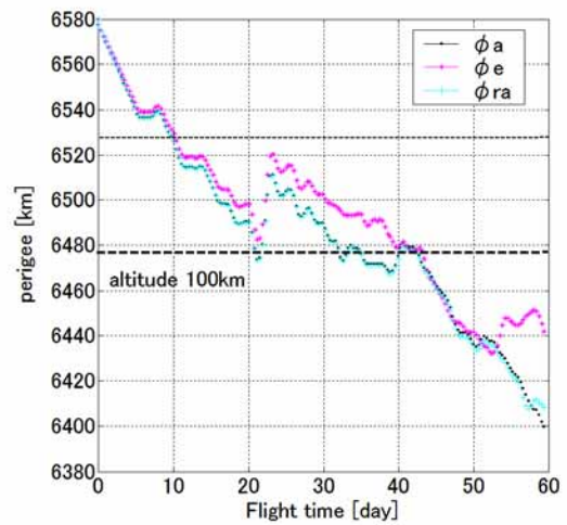
Fig.19 Change of perigee using steering law for 60 days
