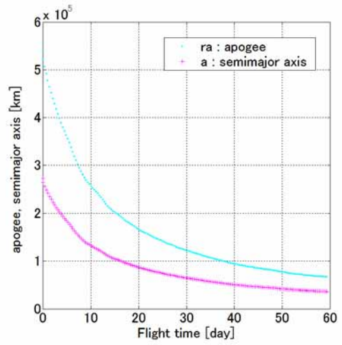
Fig.18 Change of apogee and semimajor axis using steering law for 60 days
