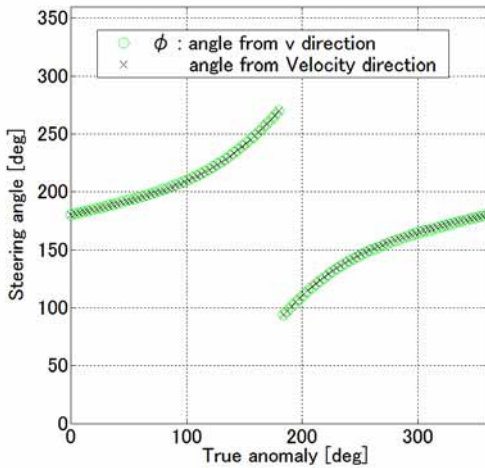
Fig.6 Optimum thrust steering angle profile
