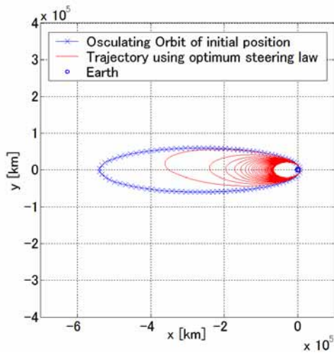
Fig.16 Trajectory using steering law for 60 days
