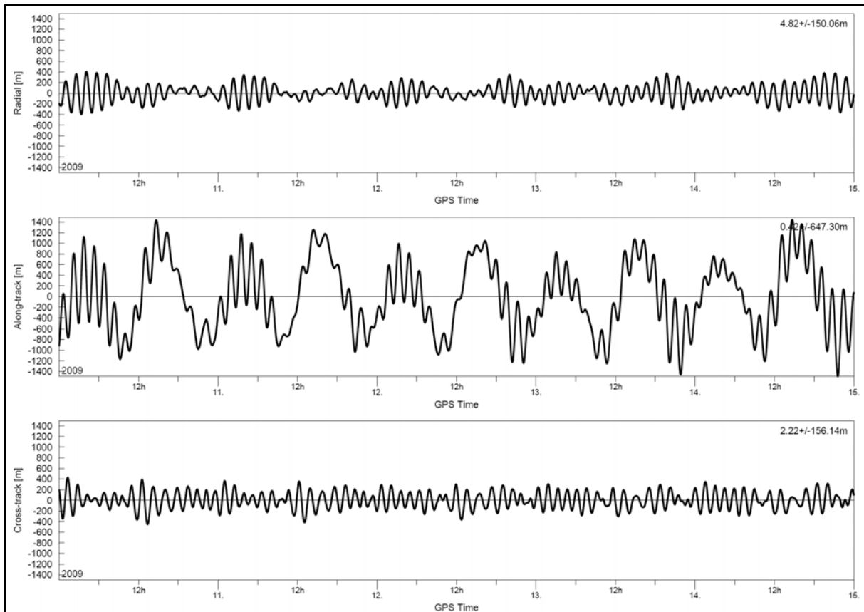
Fig. 1 RTN (radial/tangential/normal) error of a 5-days-TLE-fit w.r.t. numerically propagated orbit
