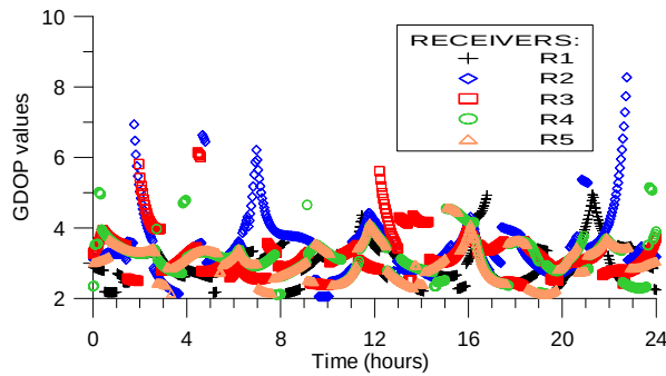
Figure 7. GDOP for Constellation 2 (14 satellites)
