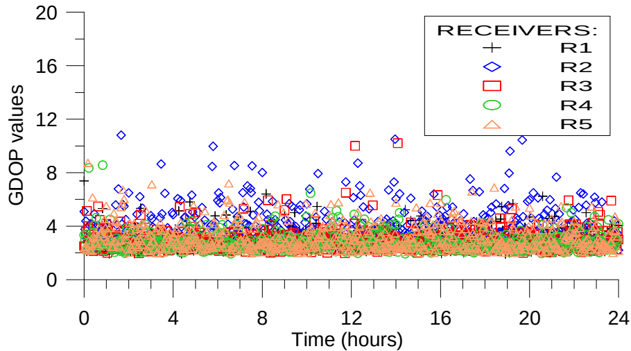
Figure 2. GDOP for Constellation 1 (140 satellites)
