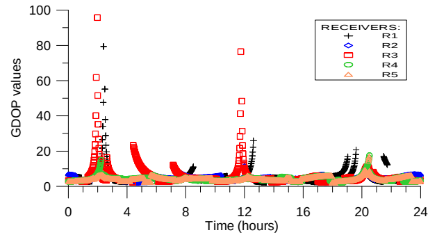
Figure 6. Zoom of Fig. 5.
