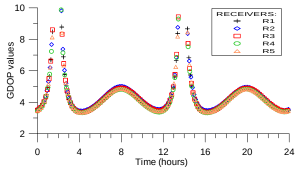
Figure 10. Zoom of Fig. 9.
