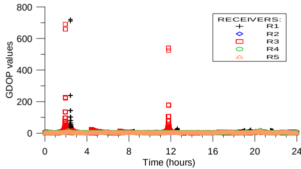
Figure 5. GDOP for Constellation 2 (12 satellites)
