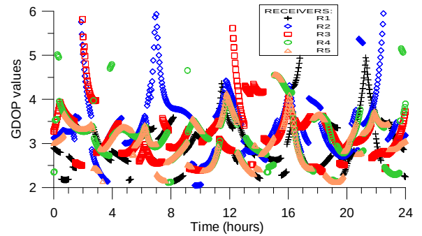
Figure 8. Zoom of Fig. 7.
