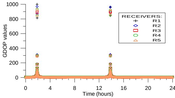
Figure 9. GDOP for Constellation 3 (4 satellites)
