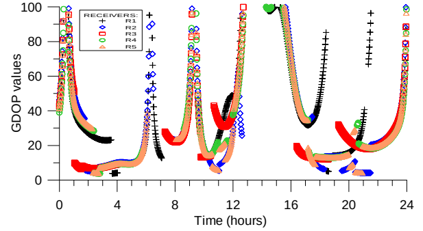
Figure 4. Zoom of Fig. 3.
