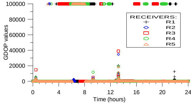
Figure 3. GDOP for Constellation 2 (10 satellites)
