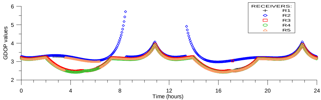
Figure 11. GDOP for Constellation 3 (5 satellites)
