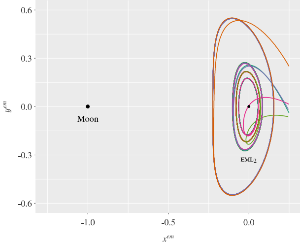
Fig. 6.: Focus on the lunar region in NCSE coordinates for the results of Figure 5, and with an identical color code. The lunar radius is not to scale.
