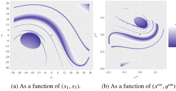
Fig. 4.: The minimum distance of projection d_p^m for t_0 = 0.99T , where T is the period of the Sun-Earth-Moon system. Only the points for which d_p^m < 10^{-2} are plotted. The symbol \bullet locates EML 2 on the two plots.
